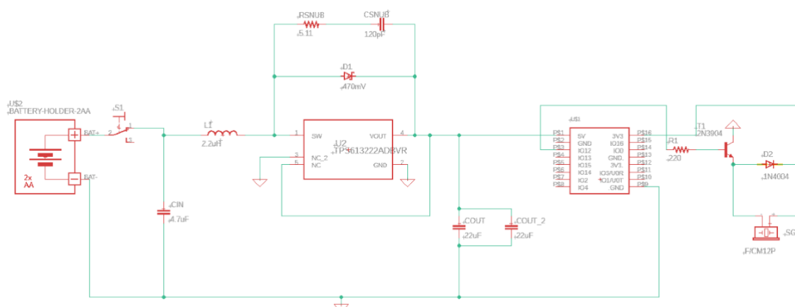
Figure 14.SD2 - Receiver's Schematic Overall
